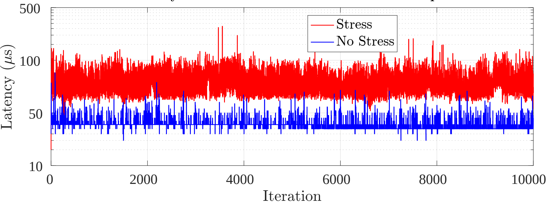
Latency for Scheduler: SCHED_DEADLINE p99
